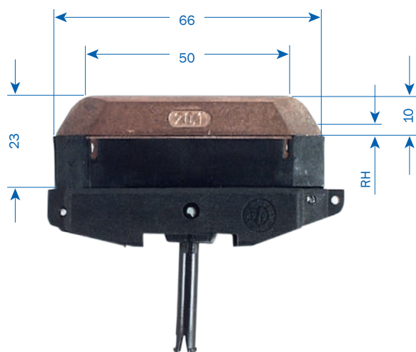
Brush KMKU 25/18 (1)
