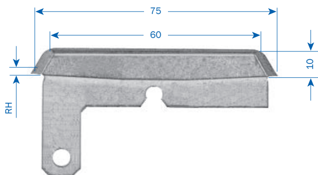
Brush KMKU 25/18 (1)
